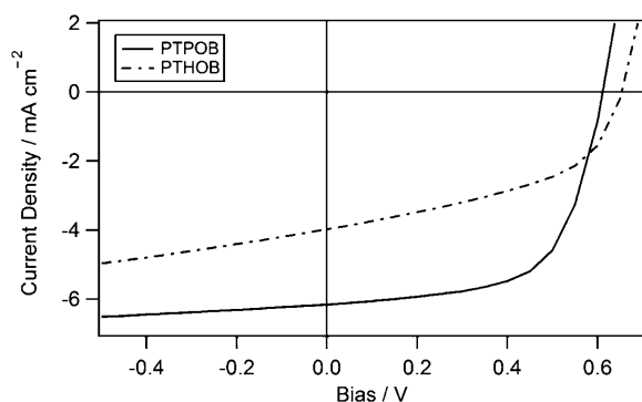
Figure 3. J - V curves of solar cells fabricated with PTPOB/P3HT in a 1:1 ratio and PTHOB/P3HT in a 1.1:1 ratio.
