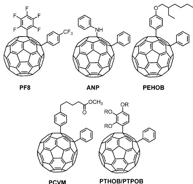
Scheme 2. Structure of some of the 1,4-addends synthesized and studied. R = propyloxy or hexyloxy.
