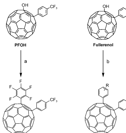
Scheme 1. Synthesis of the derivatives from fullerenols. a) Pentafluorobenzene, TsOH, 70 °C, 12 h. b) Substituted benzene (trialkylxybenzene, 2-ethylhexylbenzene, phenylvaleric acid methylester, aniline, anisole), TsOH, 80 °C, 12 h.
