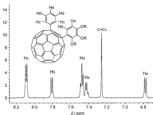
Figure 2. 1 H NMR spectrum of PTHOB. R = hexyloxy.
